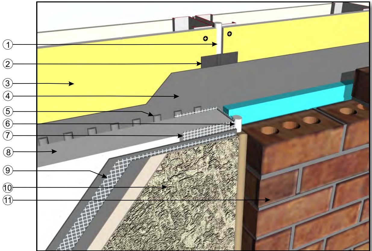
VERTICAL EXPANSION JOINT AT DISSIMILAR CLADDING
