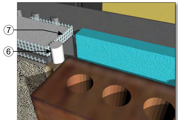
VERTICAL EXPANSION JOINT AT DISSIMILAR CLADDING
